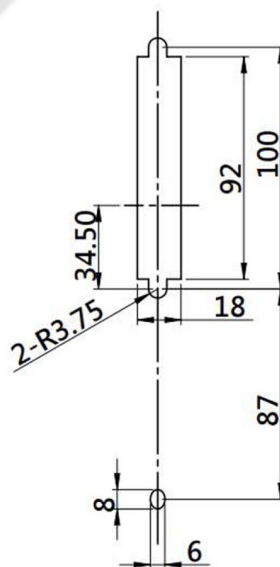
PANEL CUTOUT
